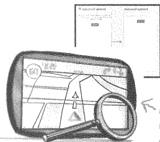
Navigation Graph
