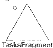
TasksFragment
